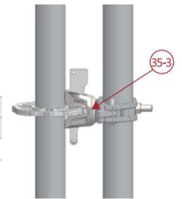
35-3. Wedge-Head Coupler Vertical
