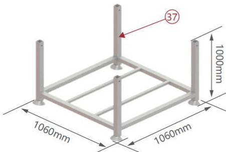
37. Scaffold Rack
