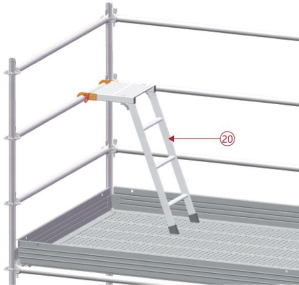
20. Aluminum Scaffolders Step
